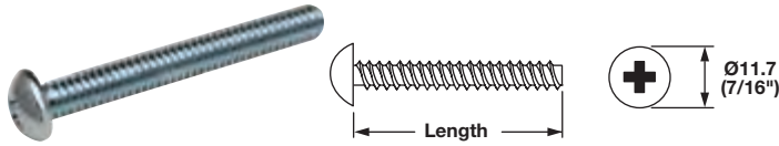
Screw, M6 With #2 Phillips Drive. Material: Steel; Finish: zinc-plated
