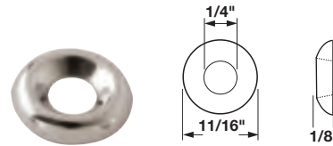
Cup Washer Used when hanging cabinets to keep screw head from pulling through panel. For #12 Countersunk Screws. Material: Steel
